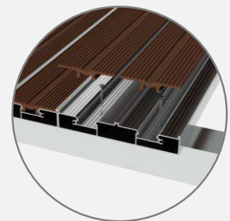
Deck + Deck Cover (Anti-Slip Cover) (Concealed Screw Fastening)
