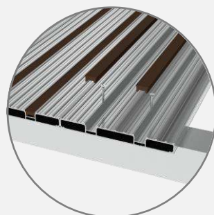
Bolt Cover Installation (Concealed Screw Fastening)
