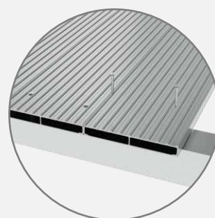
Direct Screw Fastening (Exposed Screw Fastening)
