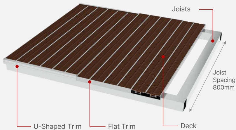
Deck + Deck Cover (Anti-Slip Cover) (Concealed Screw Fastening)
