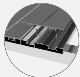
Deck + Deck Cover (Flat Cover) (Concealed Screw Fastening)
