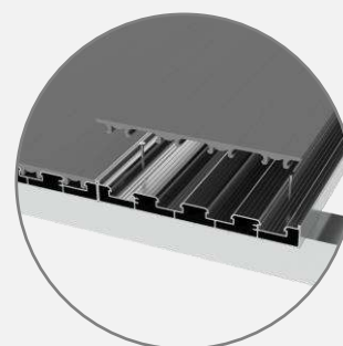
Deck + Deck Cover (Anti-Slip Cover) (Concealed Screw Fastening)
